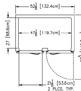
Plan View All Two Section Reach-In Models
