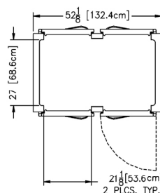
Plan View All Two Section Pass-Thru Models
