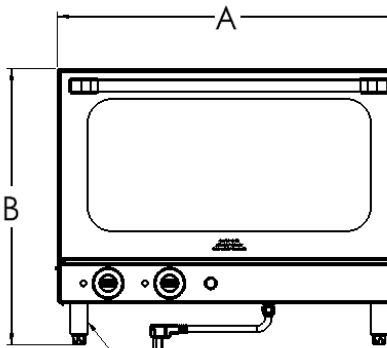
Adjustable 4" - 5" (10.2 - 12.7) legs
