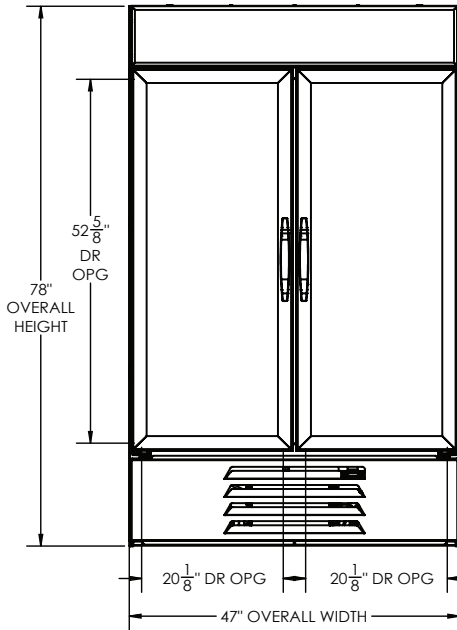
ELEVATION VIEW
