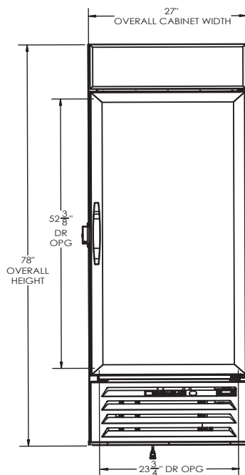
ELEVATION VIEW
