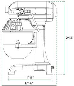
SIDE
