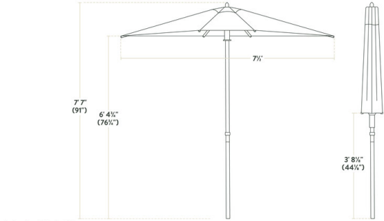
Aluminum Round Umbrella - 7' 7"
