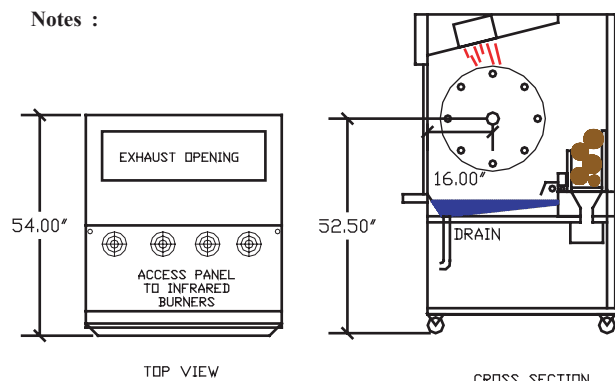
CROSS SECTION
