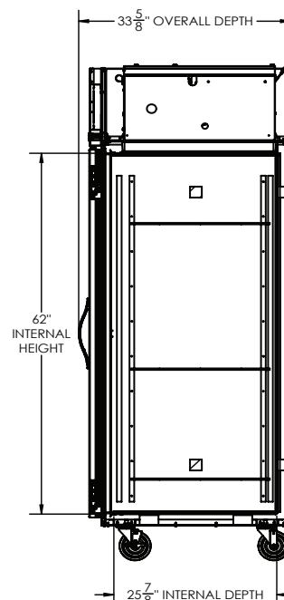
SIDE VIEW
