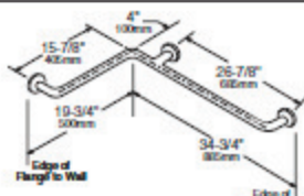
HORIZONTAL TWO-WALL BAR for Shower Stall
