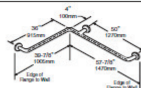
TWO-WALL WHEELCHAIR TOILET COMPARTMENT
