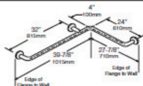
HORIZONTAL TUB / SHOWER / TOILET COMPARTMENT BAR 24 x 36
