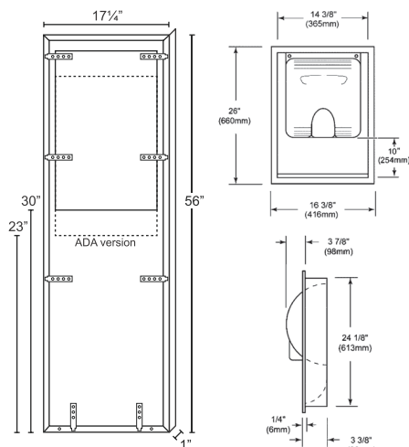
PART #40550 - STANDARD PART #40551 - ADA HEIGHT
