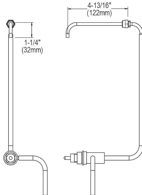
SOAP SPOUT
