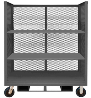
Model 3STFP-EX3048-3-6PU-95
