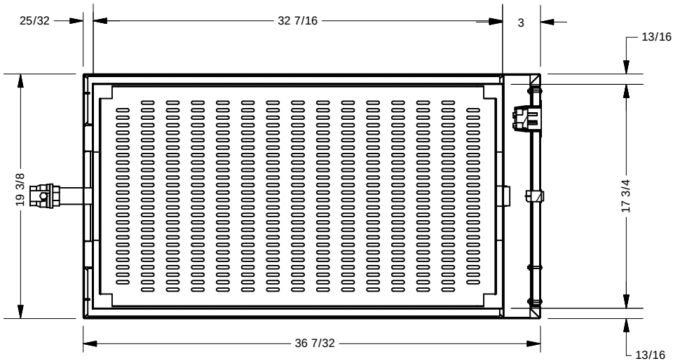
PLAN SECTION
