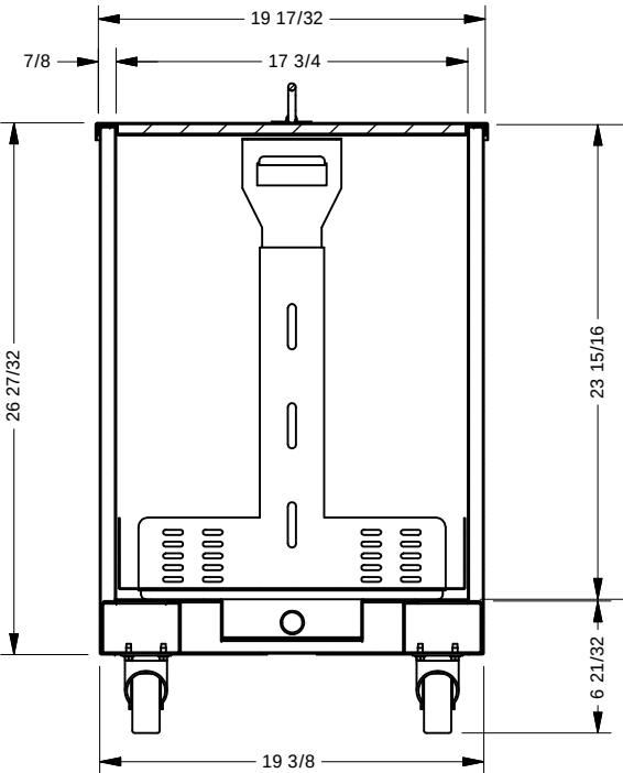
SECTION VIEW
