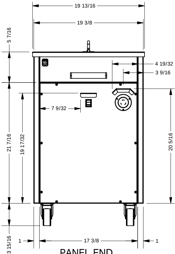
PANEL END
