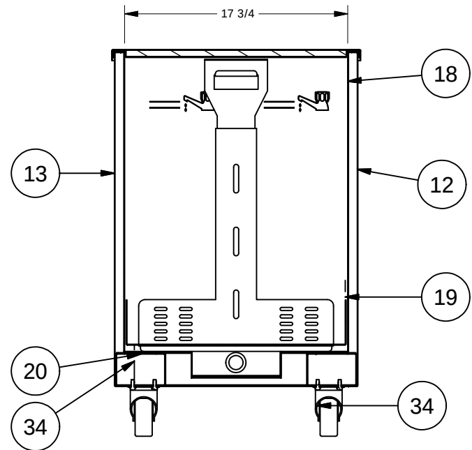
SECTION C
