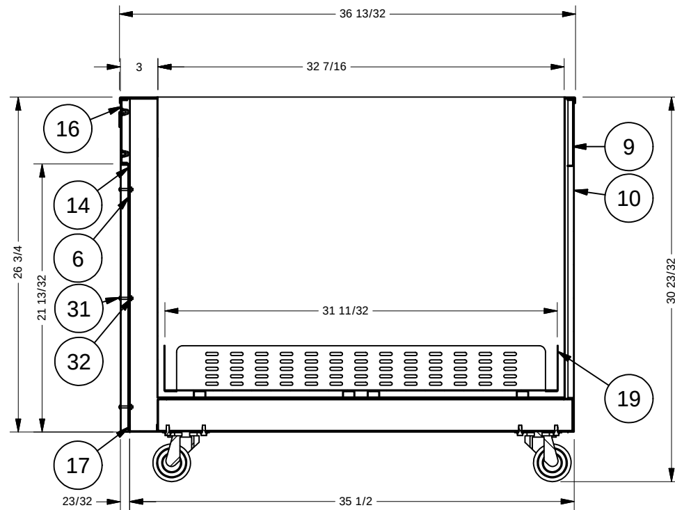
SECTION G-G W/O TOP
