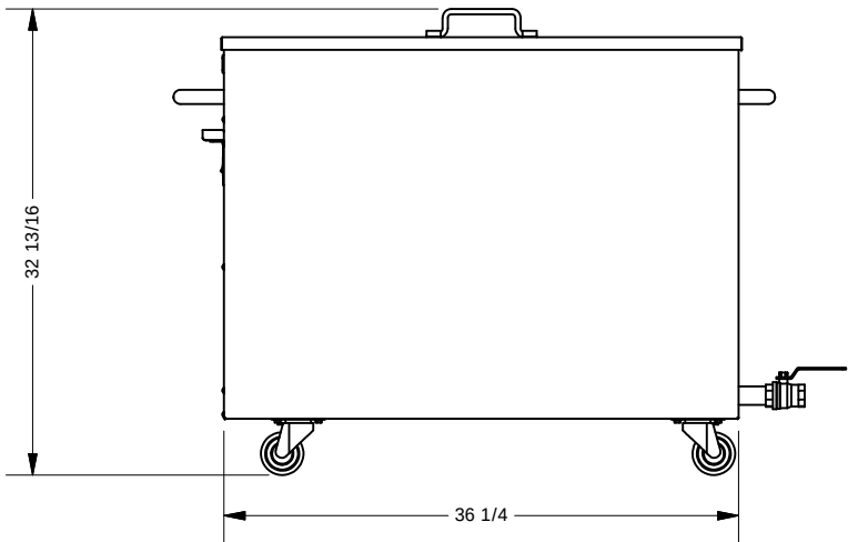
END VIEW
