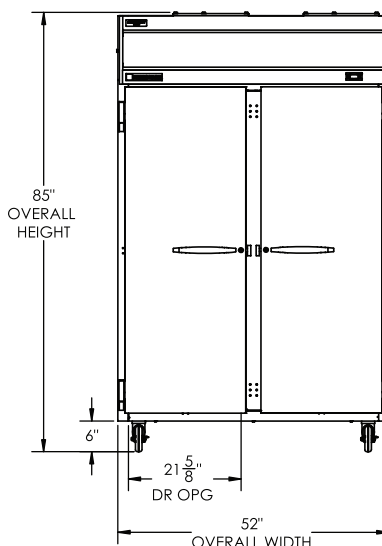
ELEVATION VIEW
