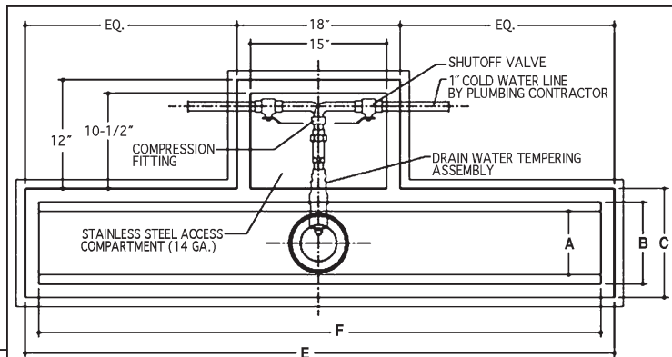
TOP VIEW of trough 18" or longer (see chart below for dimensions A through F)
