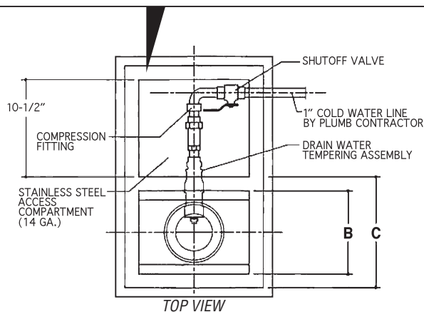
TOP VIEW of trough 18" or longer (see chart below for dimensions A through F)
