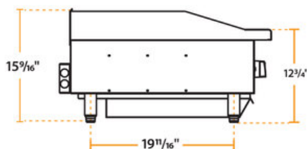
SIDE
