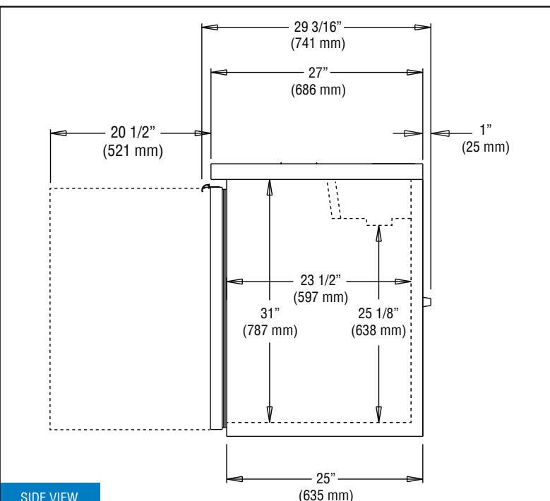
SIDE VIEW
