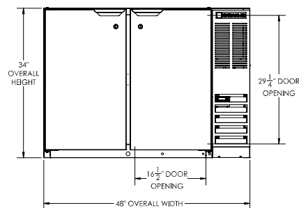
ELEVATION VIEW
