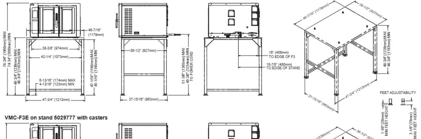
VMC-F3E on stand 5029776 with feet
