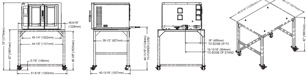
VMC-F3E on stand 5029775 with casters
