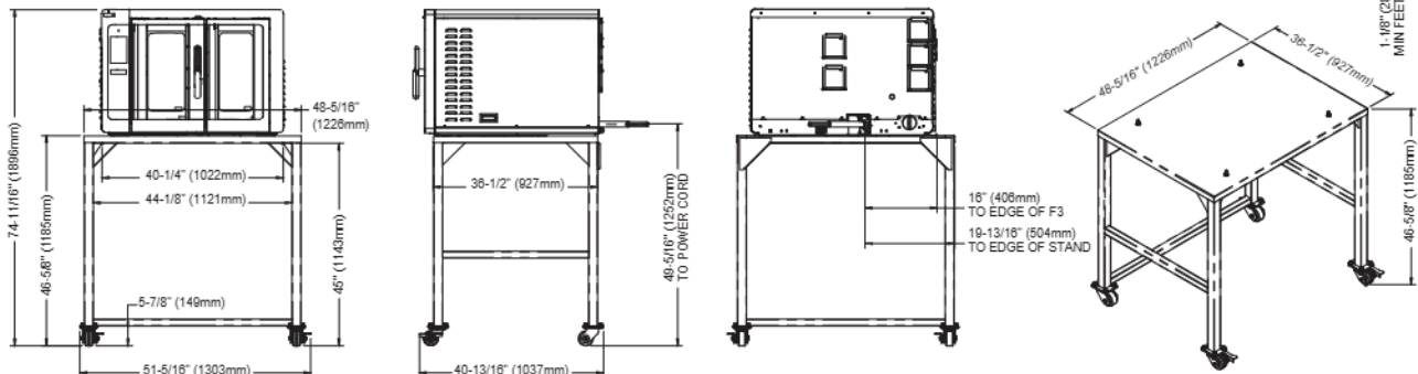
VMC-F3E on stand 5029777 with casters
