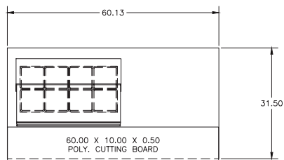
D4460NP-8 Pan Cutout Configurations
