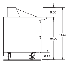
D4464NP-12M Right Side View
