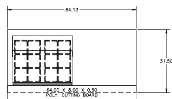
D4464NP-12M Pan Cutout Configuration
