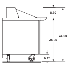
4464NP-12M Right Side View
