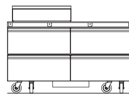
D4464NP-12M Elevation View
