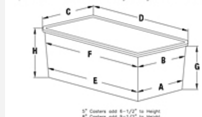
PlasticBox-Dimensions
