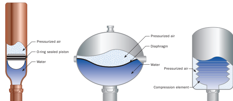
Examples of mechanical water hammer arrestors
