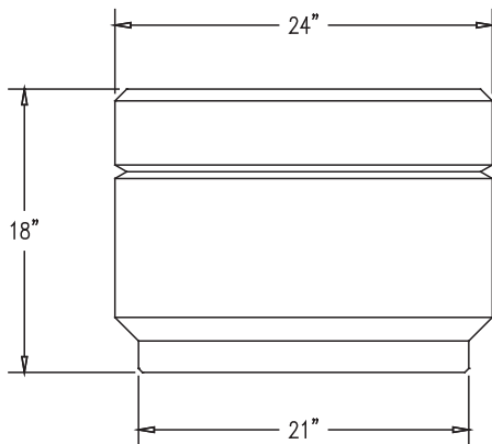
ELEVATION VIEW
