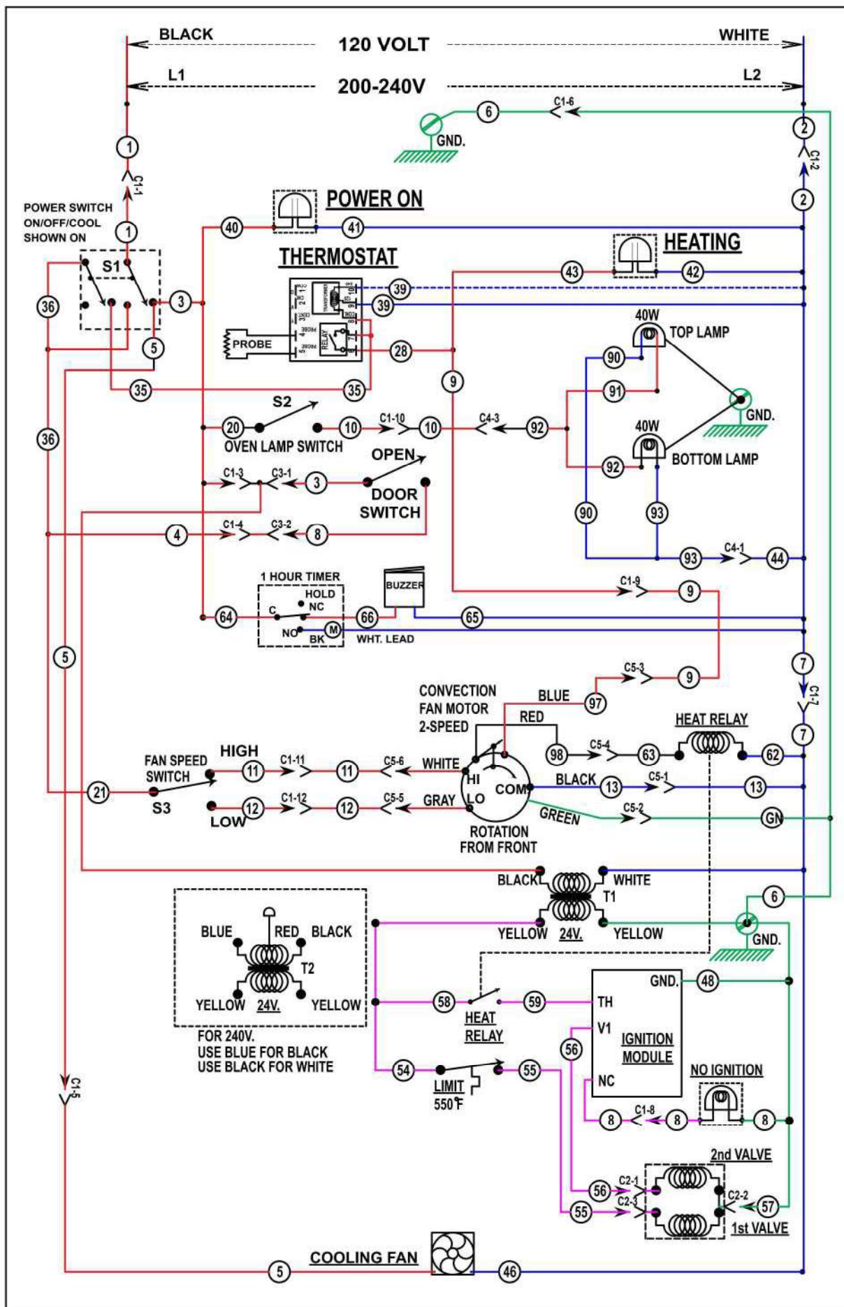
VC4 & 6GD / HGC / WKG CONVECTION OVEN STD. CONTROLS 120 TO 240V. DERIVED FROM 424299-1 Rev. D STARTING SERIAL NUMBER 481907146
