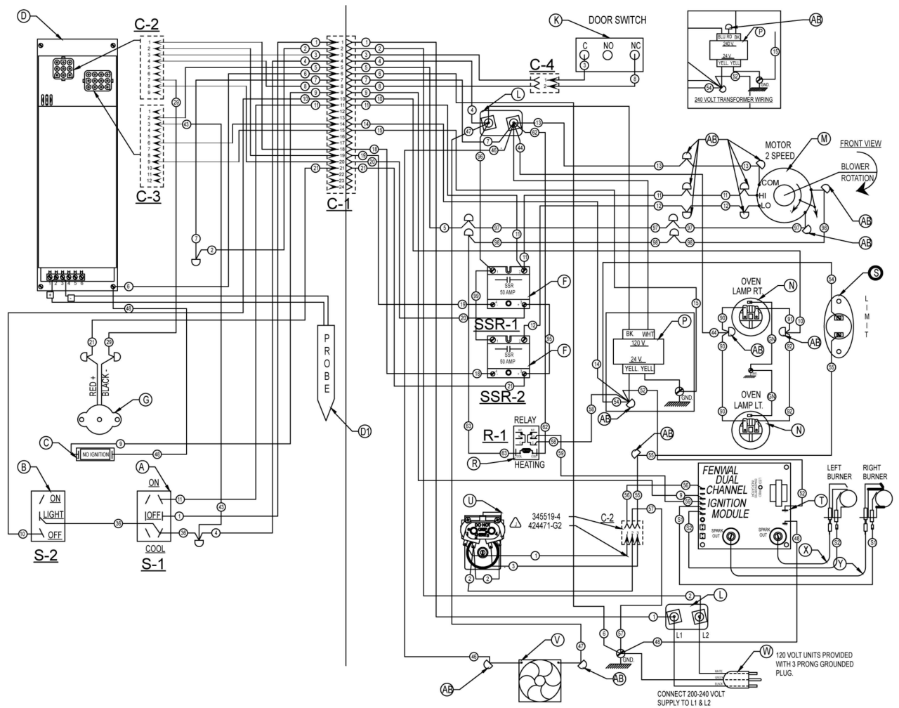
SG4 / SG6 CONVECTION OVEN DUAL BURNER - COMPUTER CONTROL 120 TO 240V. REFER TO SCHMEATIC 426575 - 1 DERIVED FROM 426574 Rev. C
