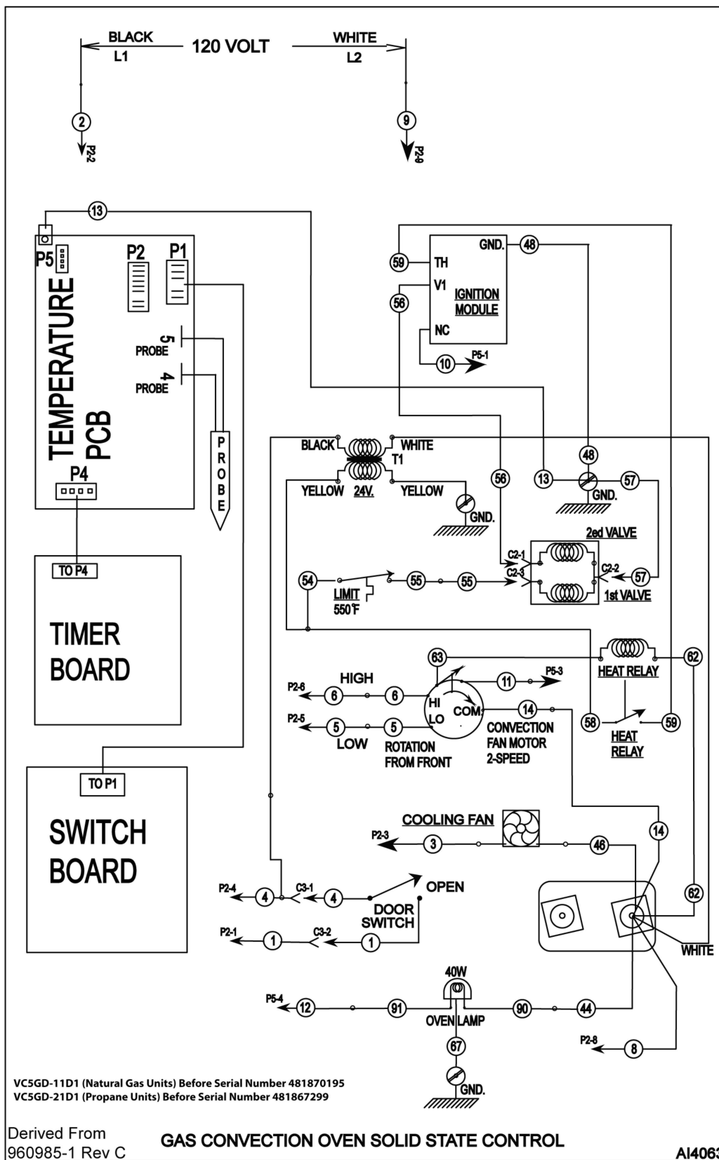
VC5GD GAS CONVECTION OVEN SCHEMATIC BEFORE SN 481870195 (Natural Gas) and 481867299 (Propane)
