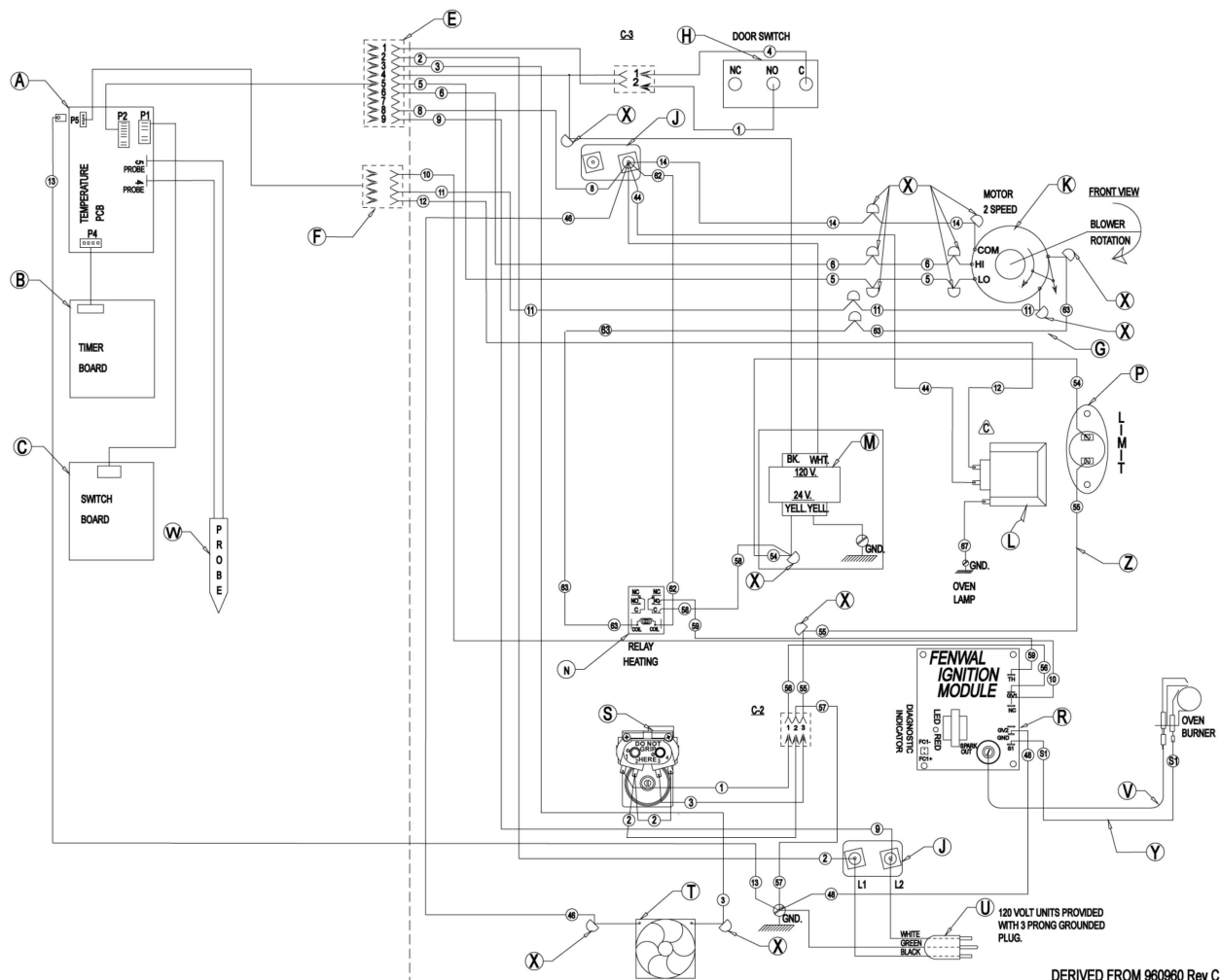
VC5GD WIRING DIAGRAM AFTER SN 481870195 (Natural Gas) and 481867299 (Propane)
