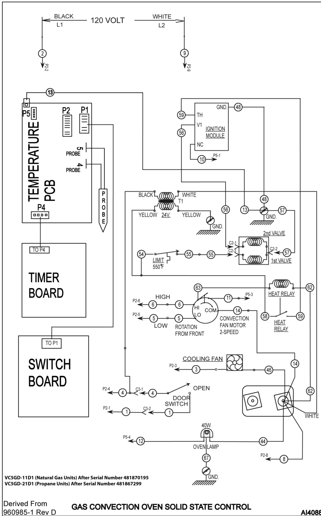
VC5GD SCHEMATIC AFTER SN 481870195 (Natural Gas) and 481867299 (Propane)
