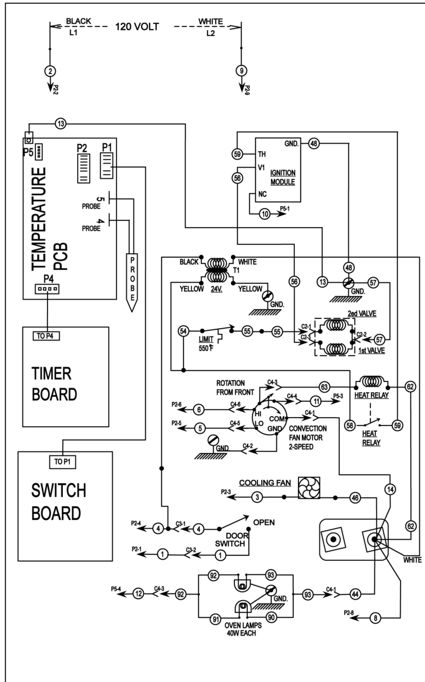
GAS CONVECTION OVEN SOLID STATE CONTROL - VC5G SCHEMATIC
