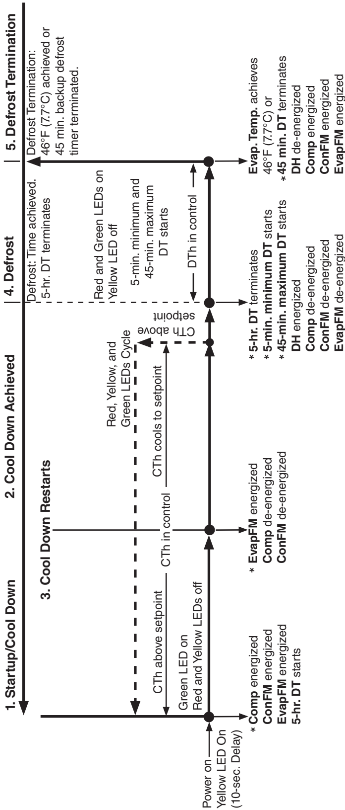
SR - Refrigerator Sequence Flow Chart
