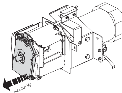
GENI, GENII & SCI blade assemblies are the same. GENII is illustrated on the left.
