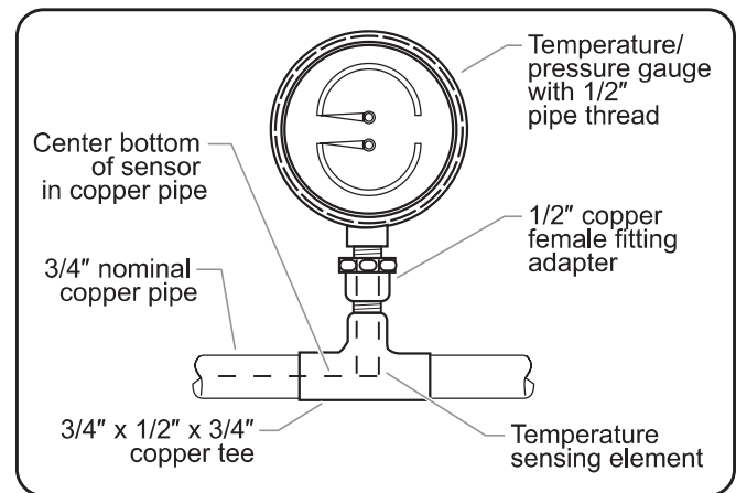
Temperature/Pressure Gauge
