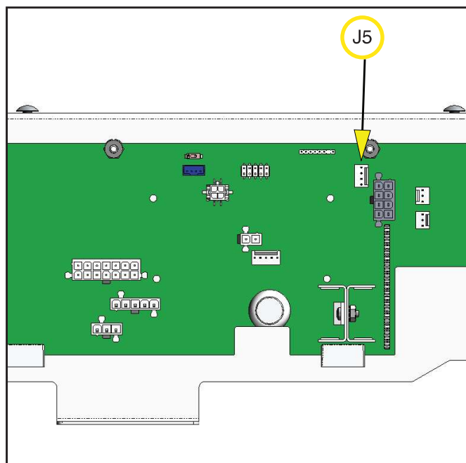
FIG. 27-3 I/O Board J5 Connector
