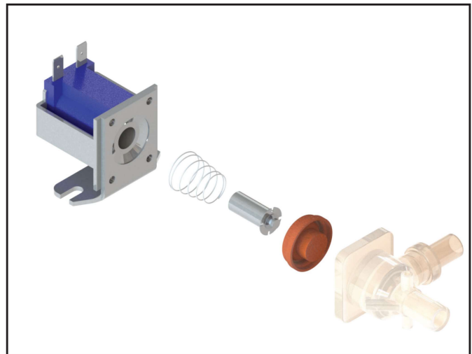
FIG. 14-2 EXPLODED VIEW
