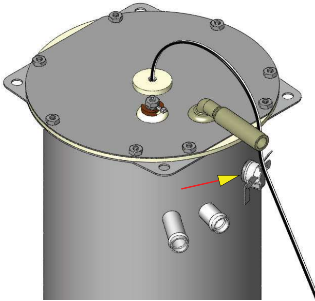
FIG. 18-1 LIMIT THERMOSTAT
