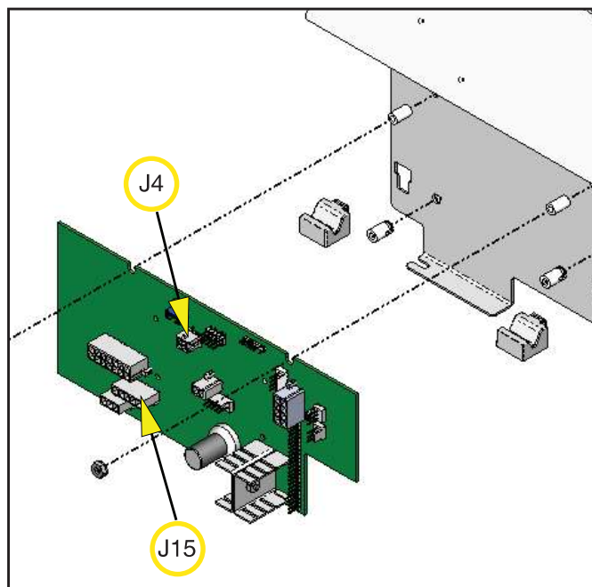
FIG. 31-2 I/O BOARD
