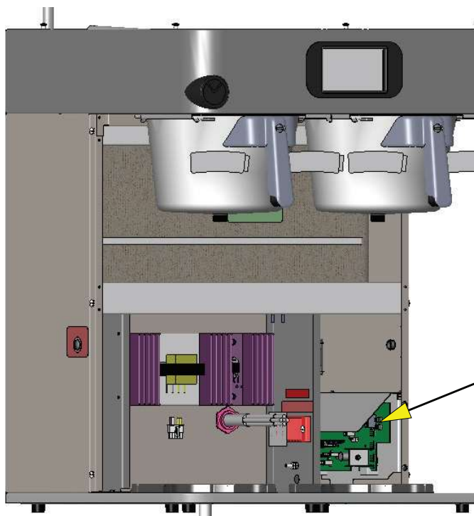
FIG. 31-1 I/O BOARD
