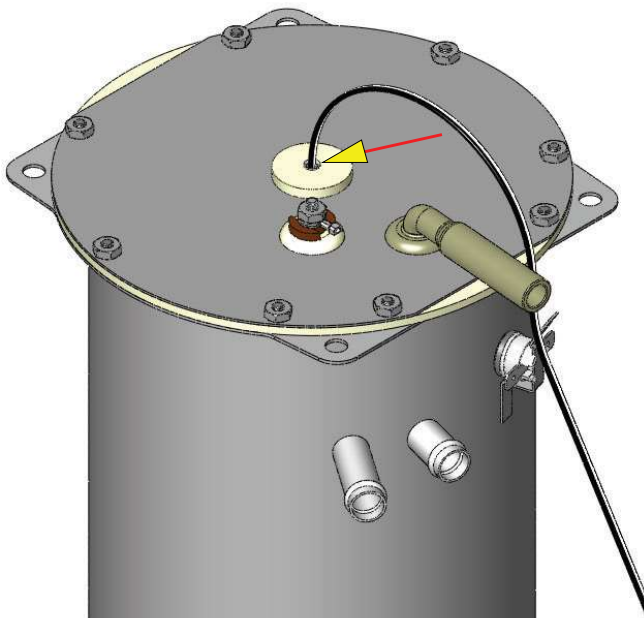
FIG. 19-1 TEMPERATURE PROBE
