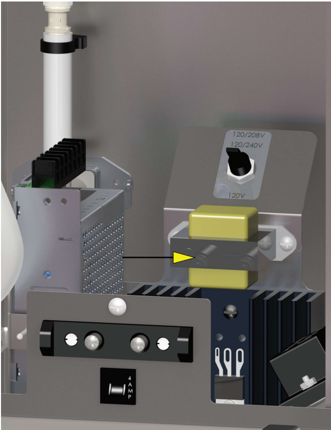
FIG. 24-1 TRANSFORMER
