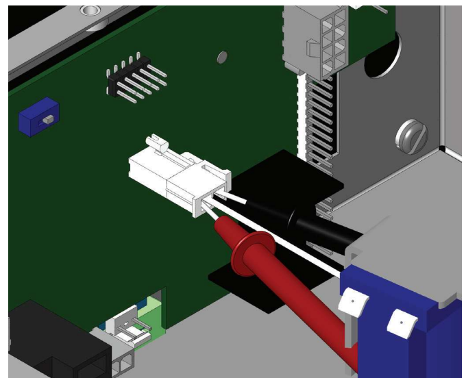
FIG. 19-3 TESTING TEMPERATURE PROBE
