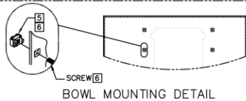
BOWL MOUNTING DETAIL
