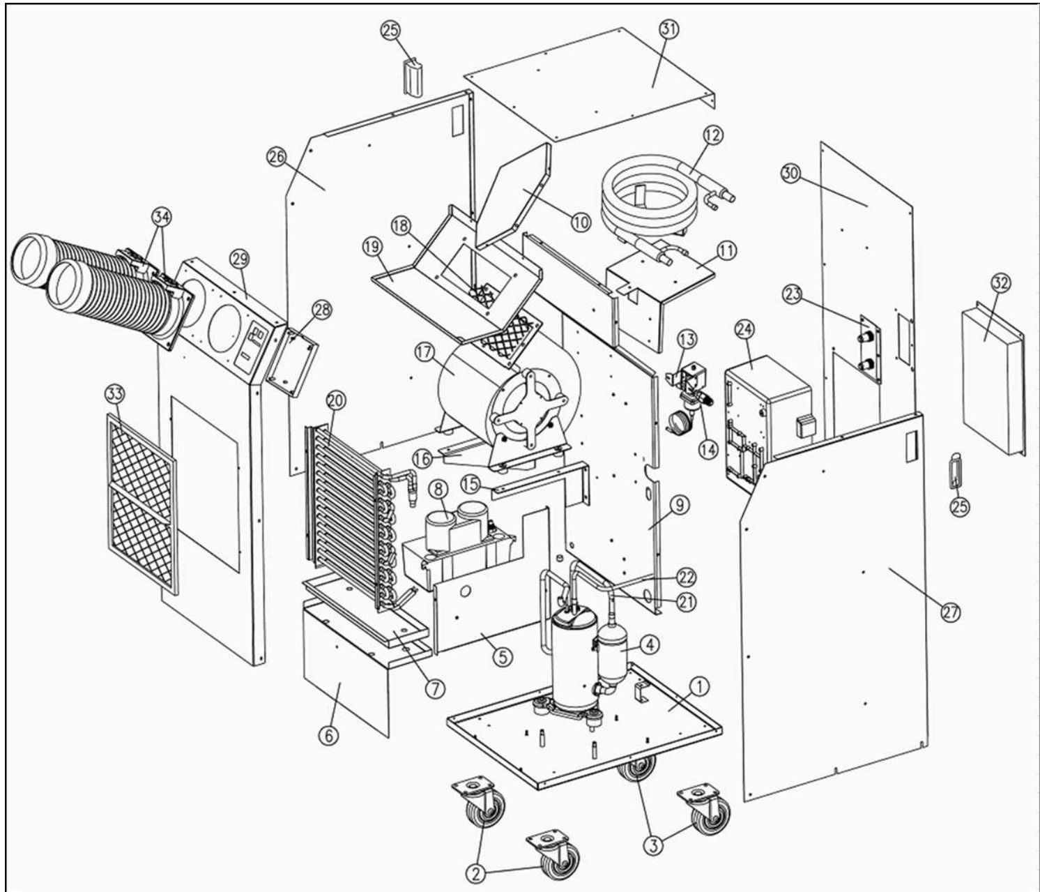
HWC-19 (수출/미국형) / ESC4001318
