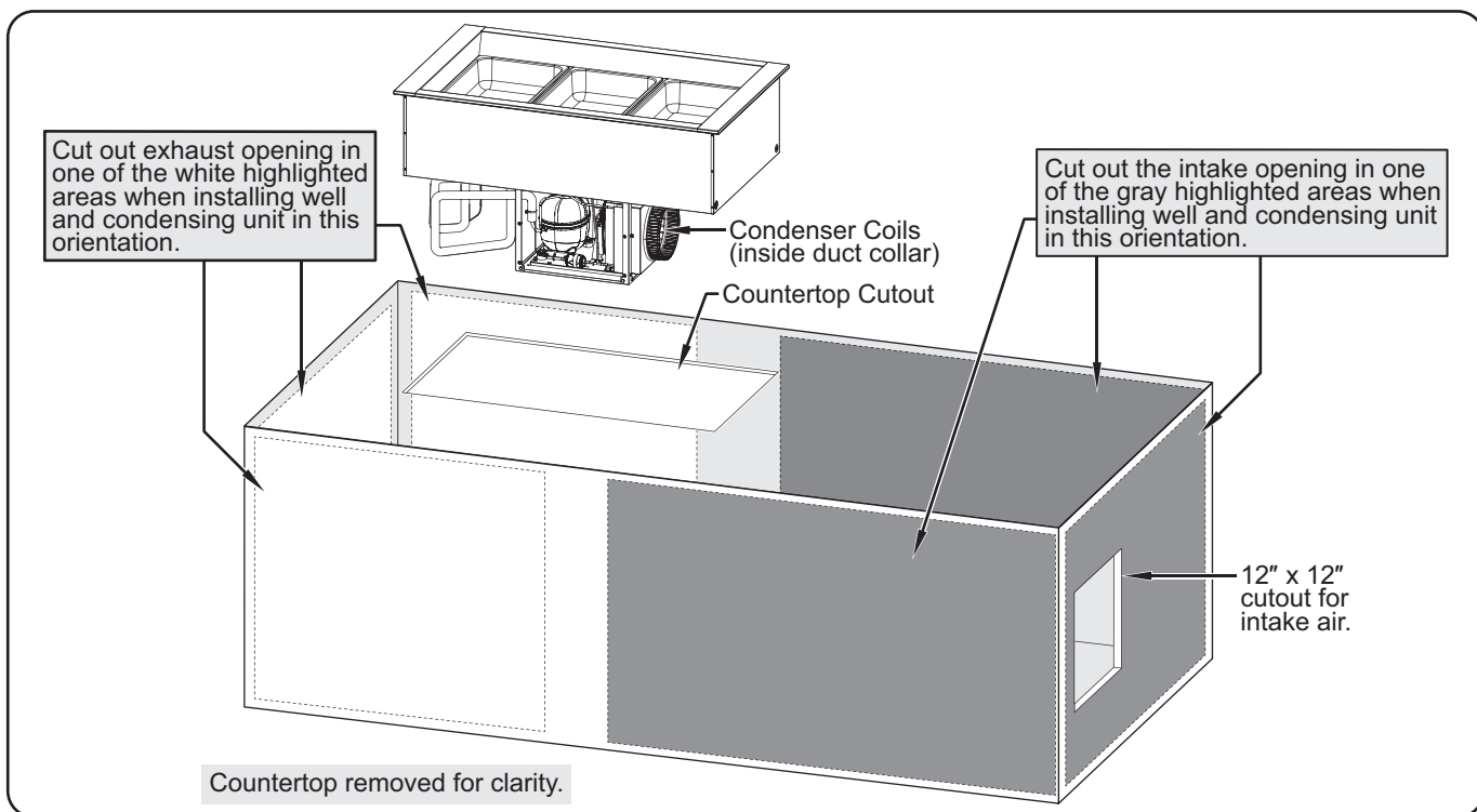
Closed Cabinet Installation (CWBP-3 Model shown)
