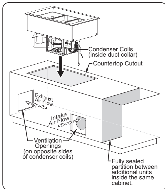
Installing a CWBP-3 Model in a Closed Cabinet
