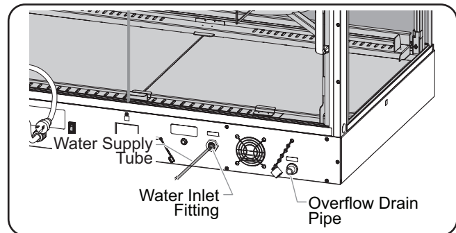
Connecting the Water Supply (IHDCH-45 shown)
