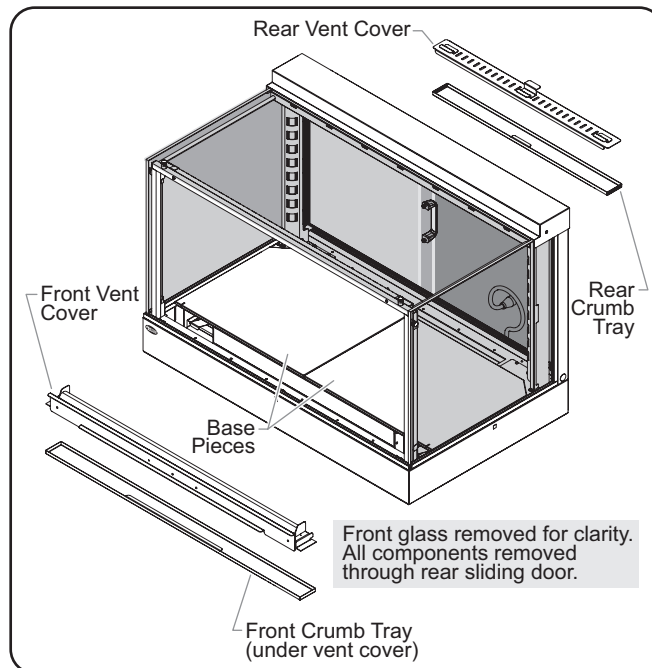
Removing/Installing Components (IHDCH-45 shown)
