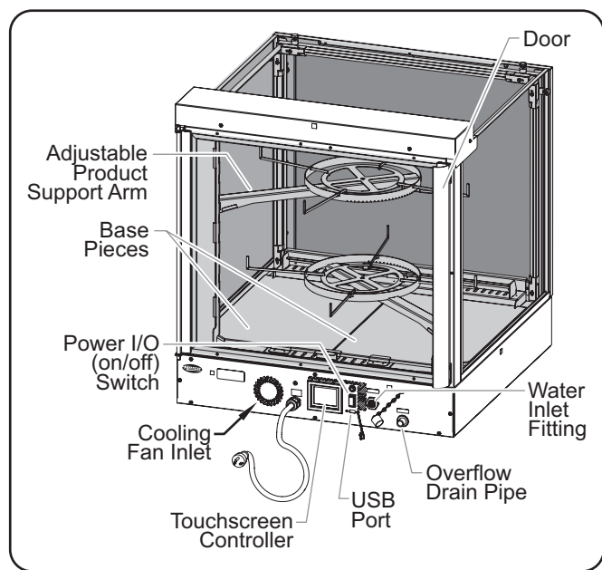
Rear view of Model IHDCH-28
