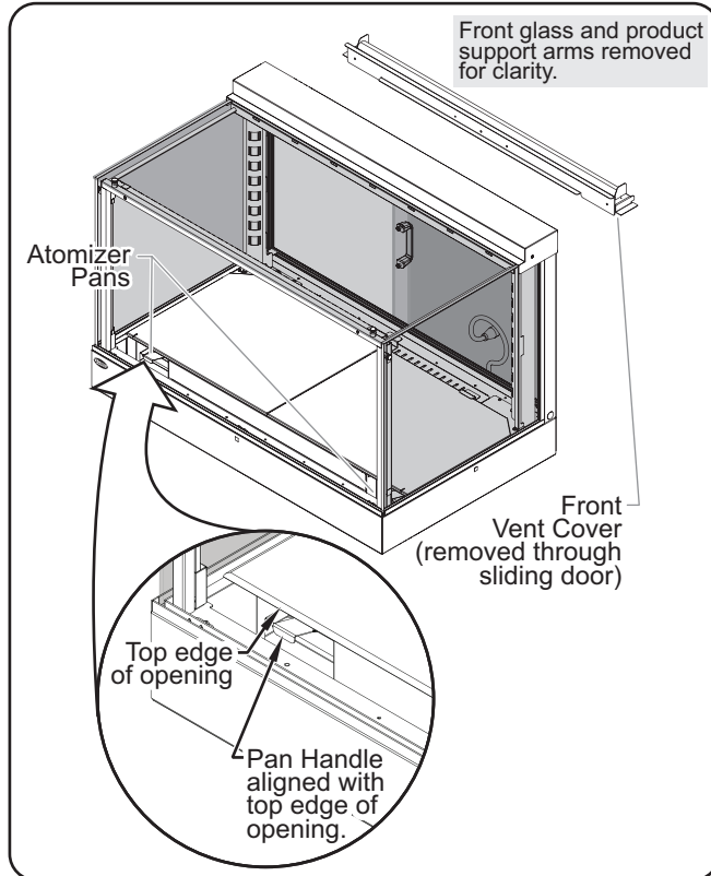
Checking the Atomizer Pans (IHDCH-45 shown)
