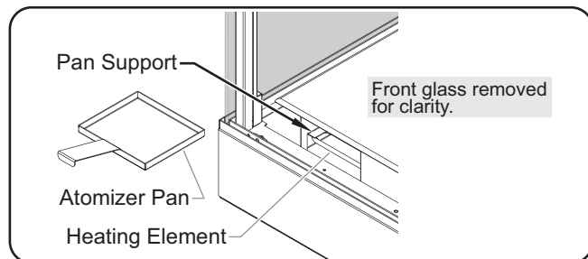
Atomizer Pan Location (IHDCH-45 shown)
