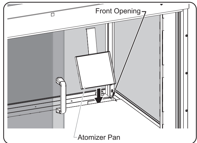
Removing/Installing the Atomizer Pans (IHDCH-45 shown)
