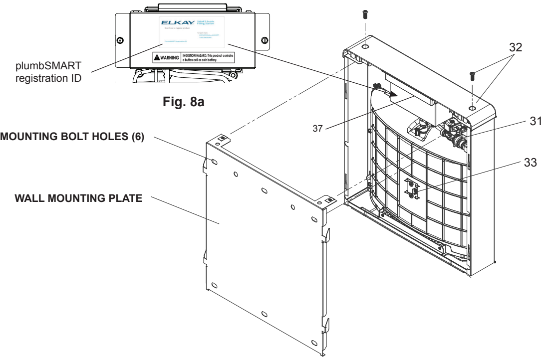
Fig. 8 BOTTLE FILLING UNIT
