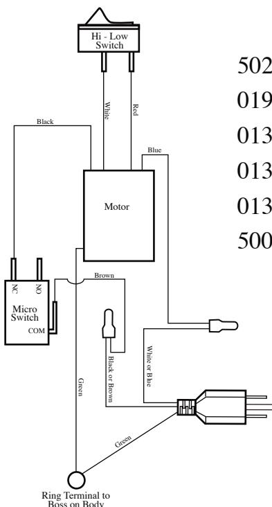
Wiring Diagram for DMC20
