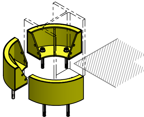
COLUMN GUARDS CAN BE MOUNTED SEPARATELY TO FIT AROUND LARGER ITEMS OR OMITTED TO AVOID OBSTACLES
