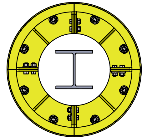
STEP 3: LAG THE COLUMN GUARD SECTIONS TO THE FLOOR USING PROVIDED ANCHORS AND SPECIFICATIONS
