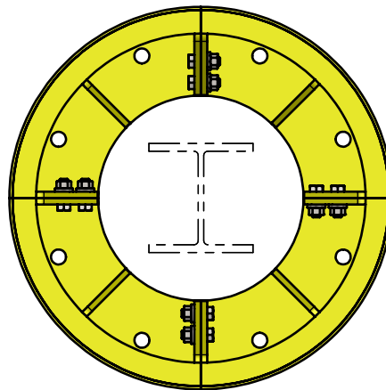
STEP 2: BOLT THE COLUMN GUARD SECTIONS TOGETHER
