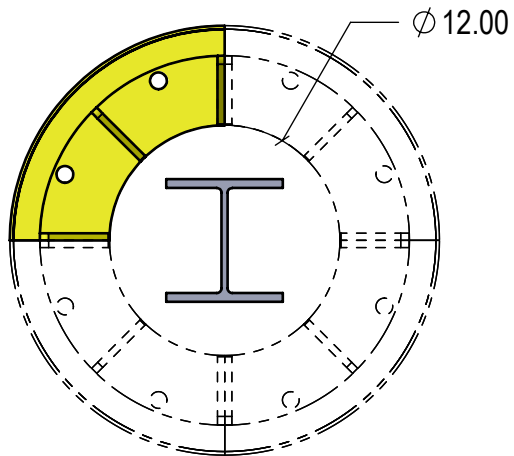
STEP 1: POSITION THE COLUMN GUARDS AROUND COLUMN
