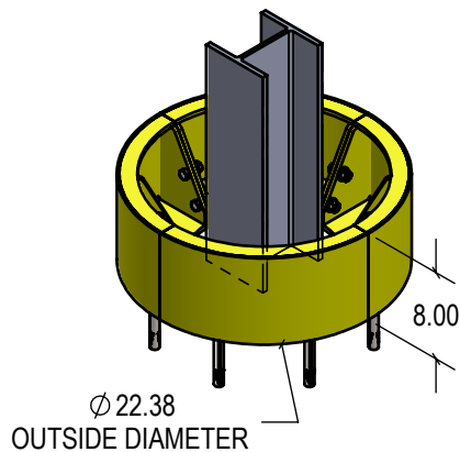
COMPLETED COLUMN GUARD INSTALLATION
