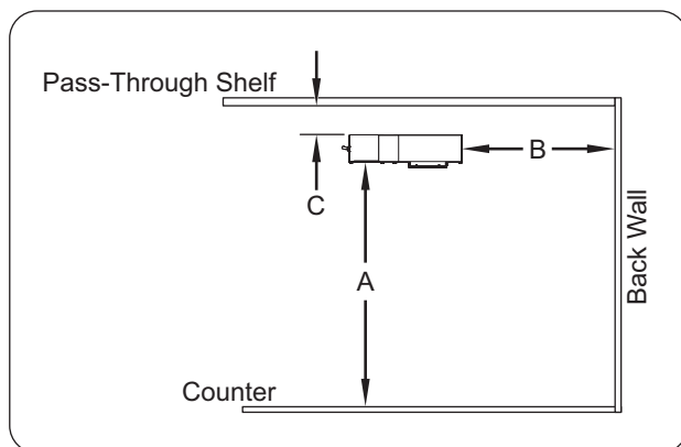
Figure 7. Clearance Requirements
