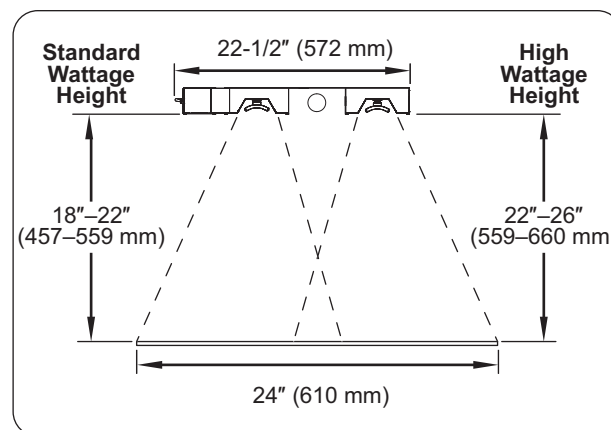
Figure 10. Recommended Mounting Height for all UGA dual element depth models with a 6" (152 mm) spacer.
