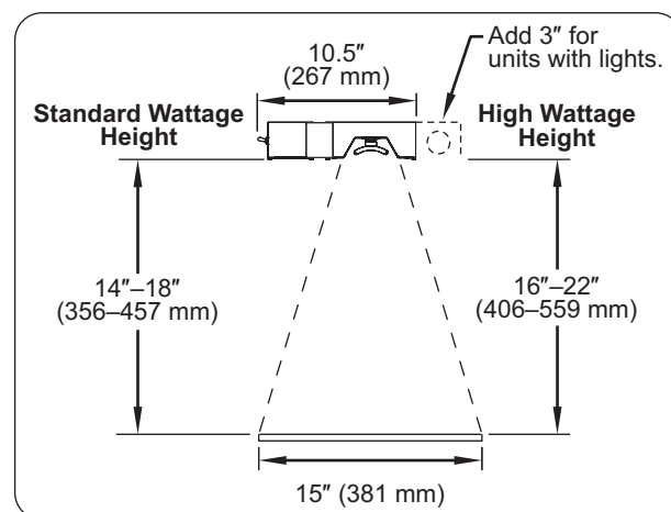
Figure 8. Recommended Mounting Height for all UGA single element depth models.
