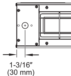
Figure 14. Countertop Conduit Hole Dimension
