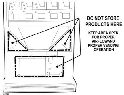
Figure 11. Refrigeration
